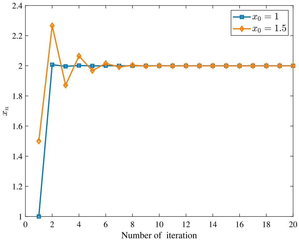
Figure 1. Iterative process of Example 4.1.
