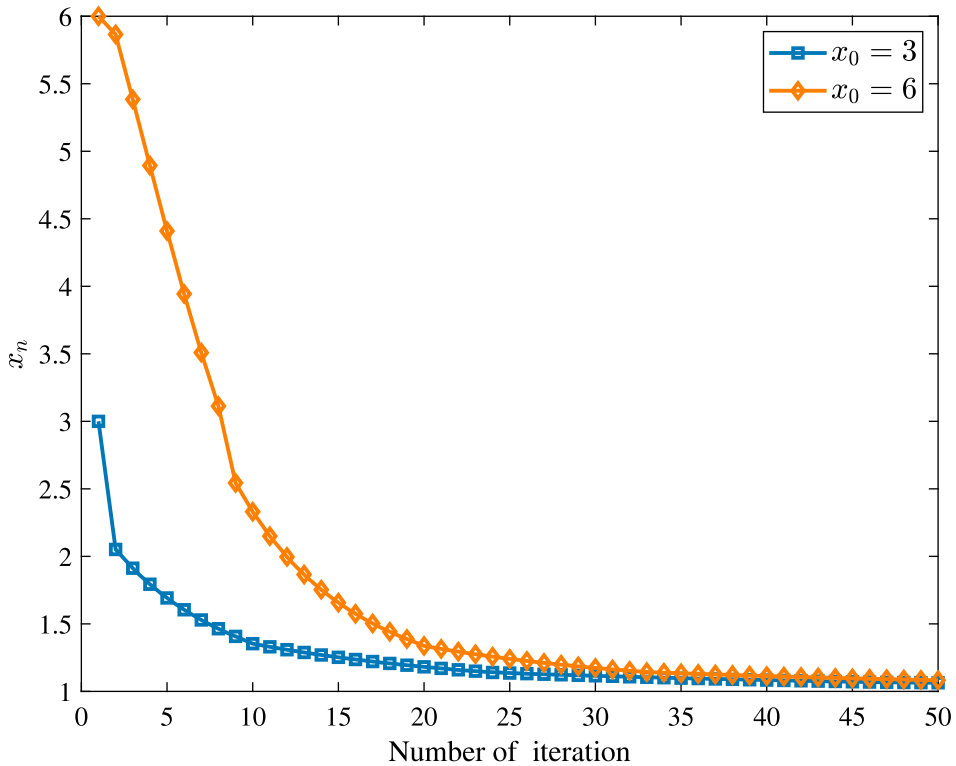
Figure 2. Iterative process of Example 4.2.
